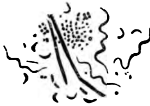
FIG. 98.— SPIRILLUM SPUTIGENUM . Occurring with spirochaeta denticola , leptothrix-filaments, micrococci, and bacteria in a scraping from a carious tooth, X 1200.
